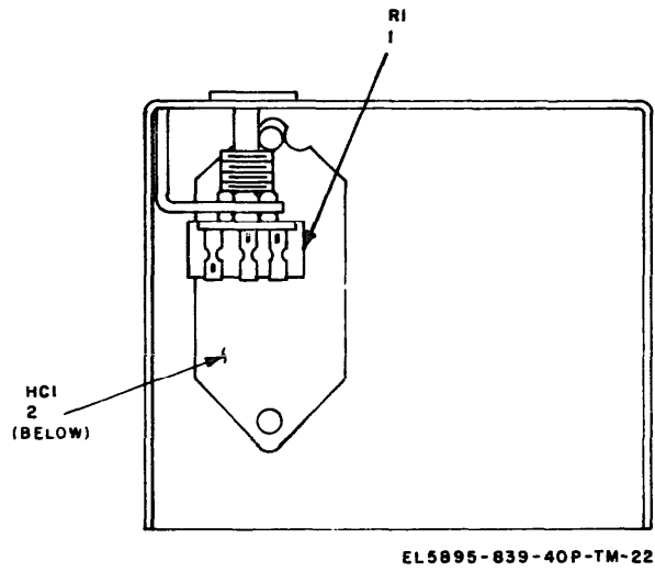
Figure 22. Power Supply PP-7147/U, front view, inside.
