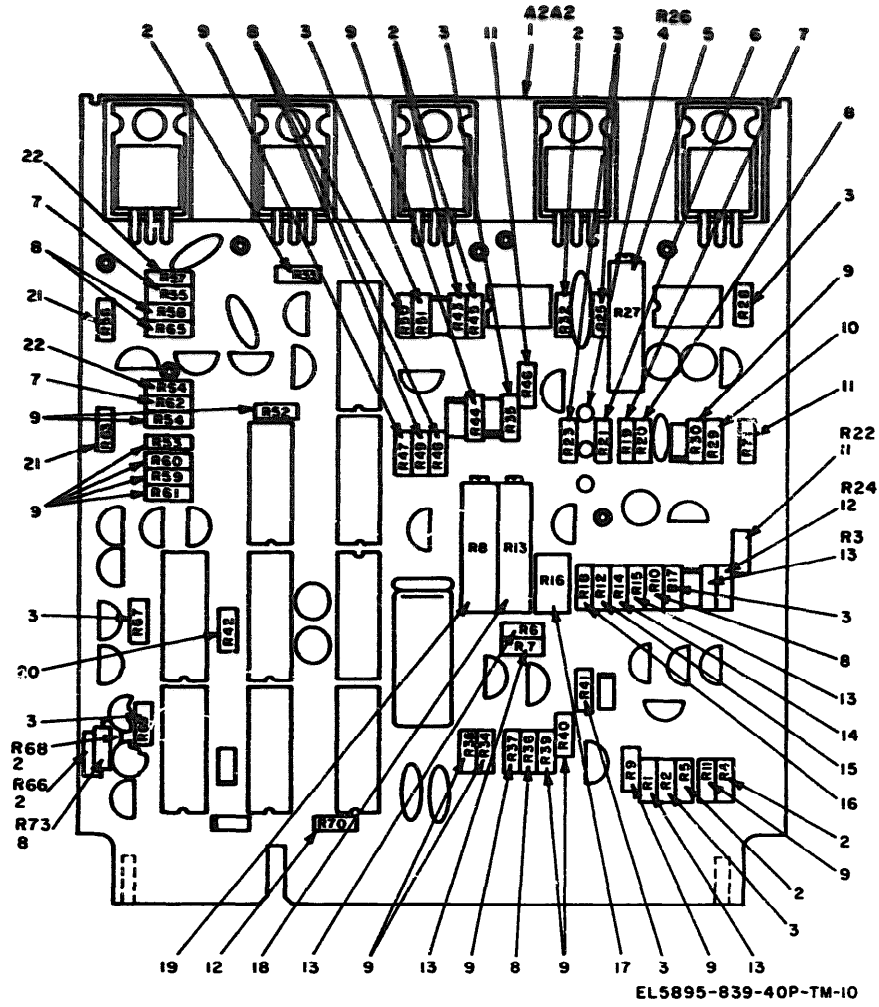
Figure 10. Circuit card assembly 85000002-001 (motion control), resistor location.
