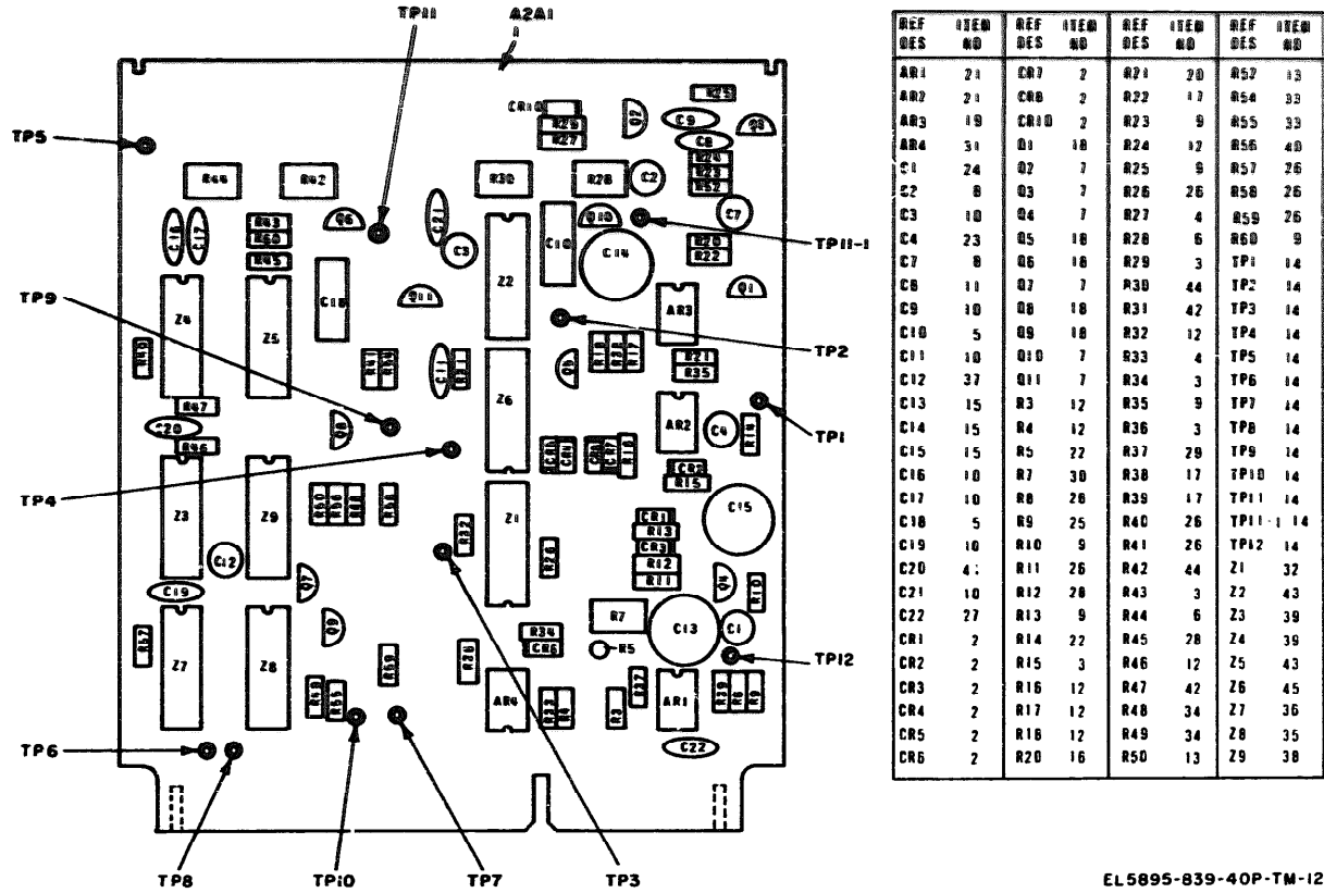
Figure 12. Circuit card assembly 8500004-001 (data electronics), parts location.
