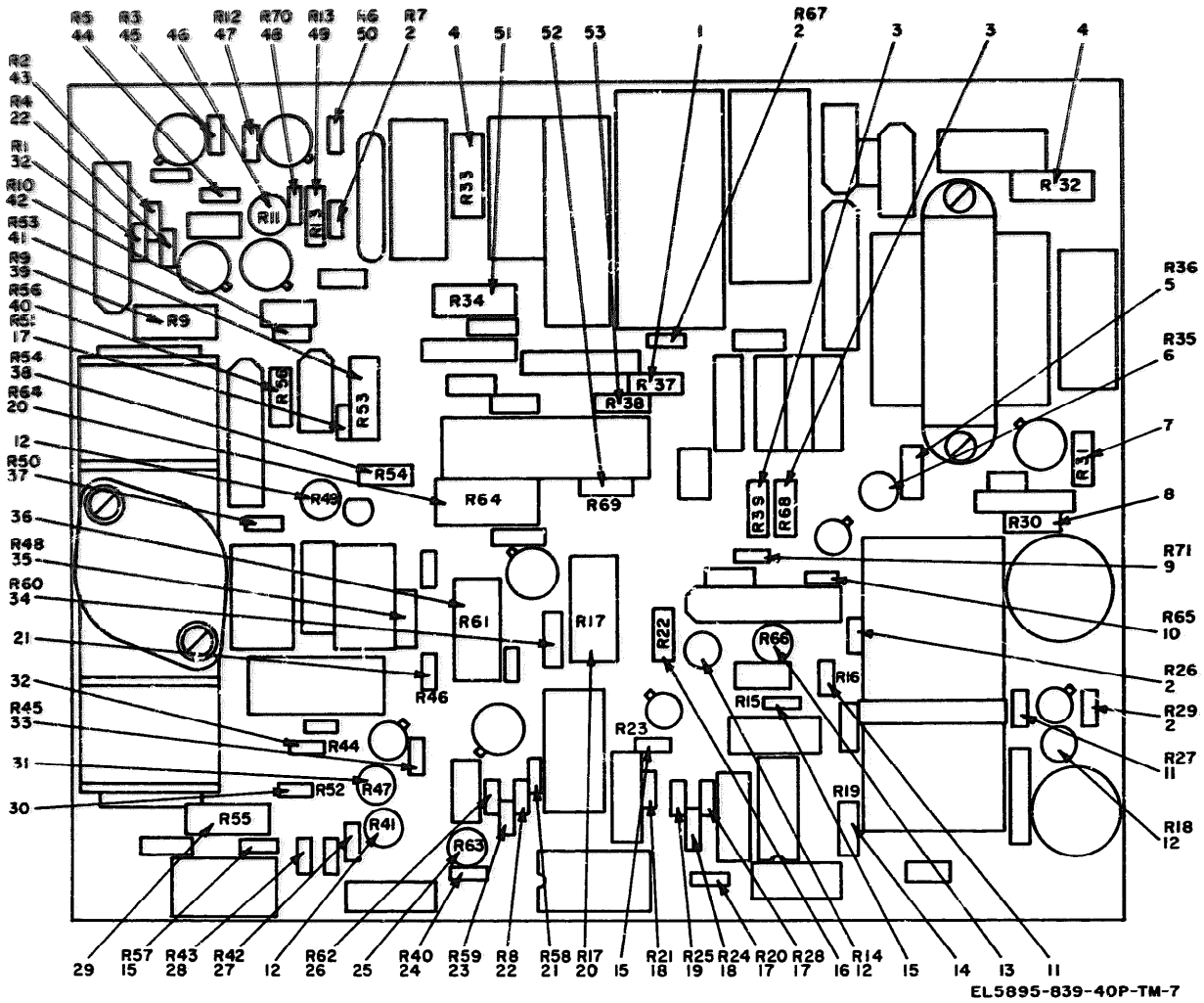
Figure 7. Circuit card assembly, 398-14939-1 (video and deflection), resistor location.
