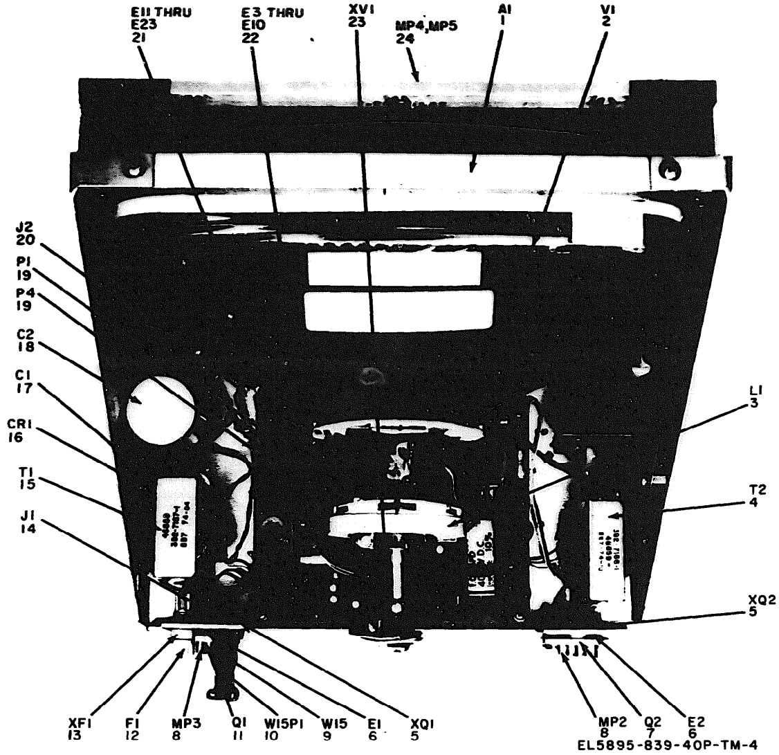
Figure 4. CRT display, 398-14937-1, parts location.
