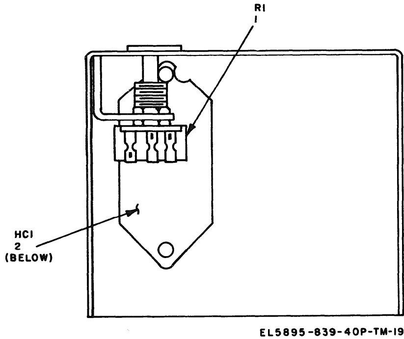
Figure 19. Power Supply PP-7145/U, front view, inside.
