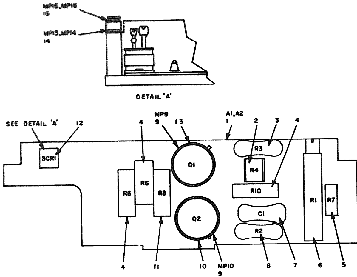
Figure 29. Voltage regulator. LMOV2, parts location.
