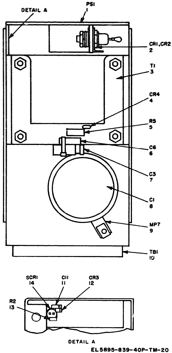
Figure 20. Power Supply PP-7147/U, top view, inside.
