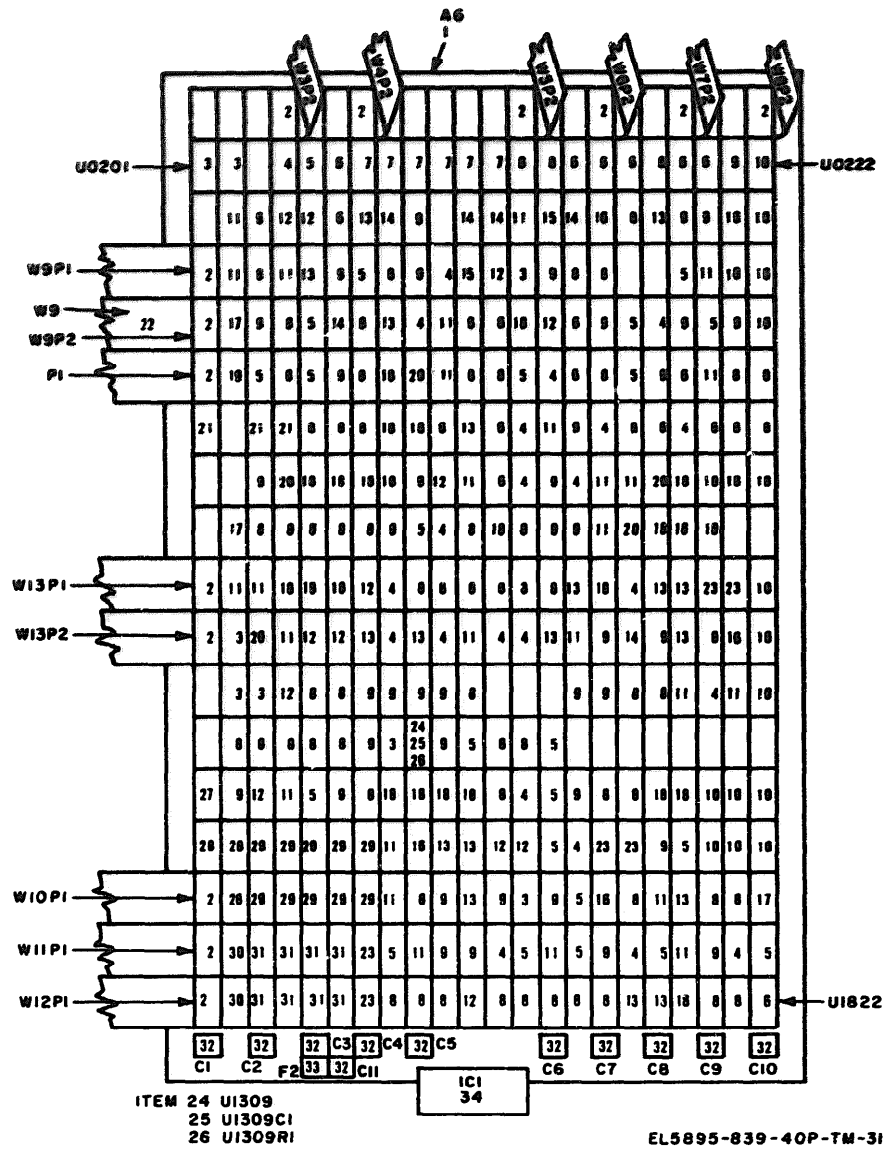
Figure 31. Interface and control logic panel, 398-15872-2, parts location.
