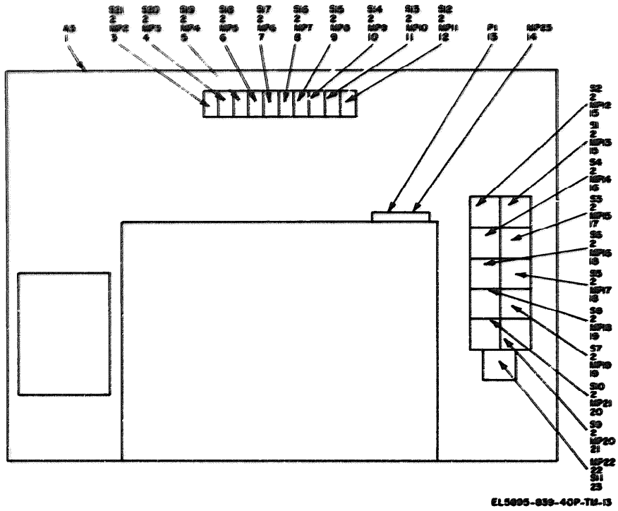
Figure 13. Keyboard assembly, 398-15369-1, parts location
