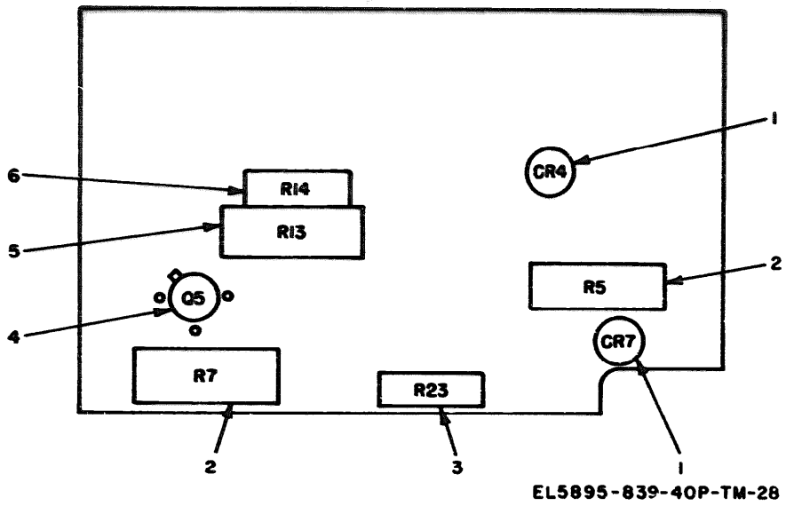
Figure 28. Power Supply PP-7144/U, component board, parts location.
