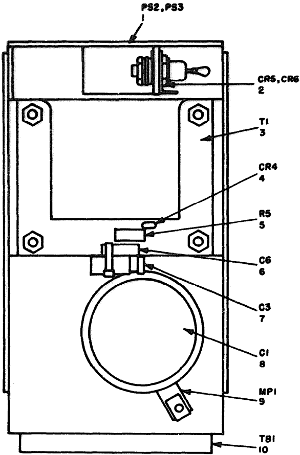
Figure 17. Power Supply PP-7145/U, top view, inside.
