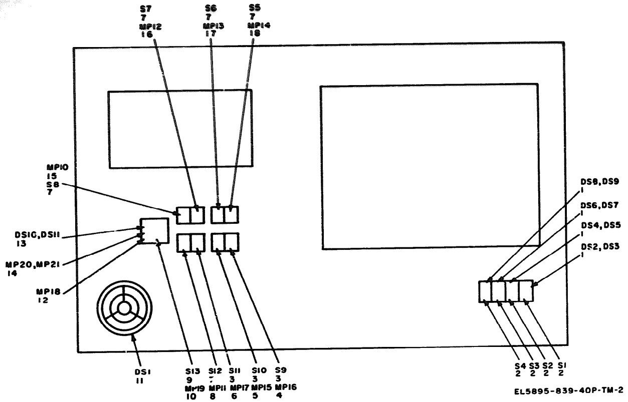
Figure 2. Message console control panel, parts location.
