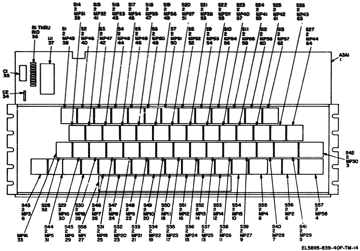
Figure 14. Keyboard subassembly 58SW5-2, parts location.
