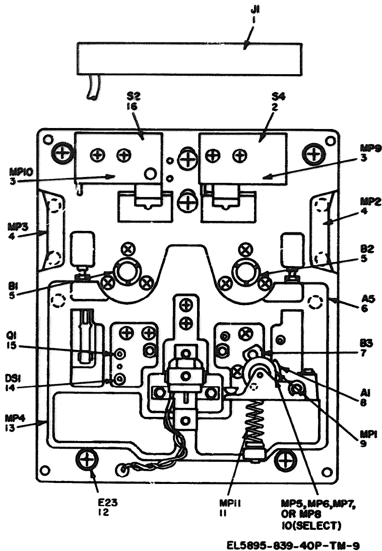
Figure 9. Tape cassette, interior view, IC2511-44, parts location.
