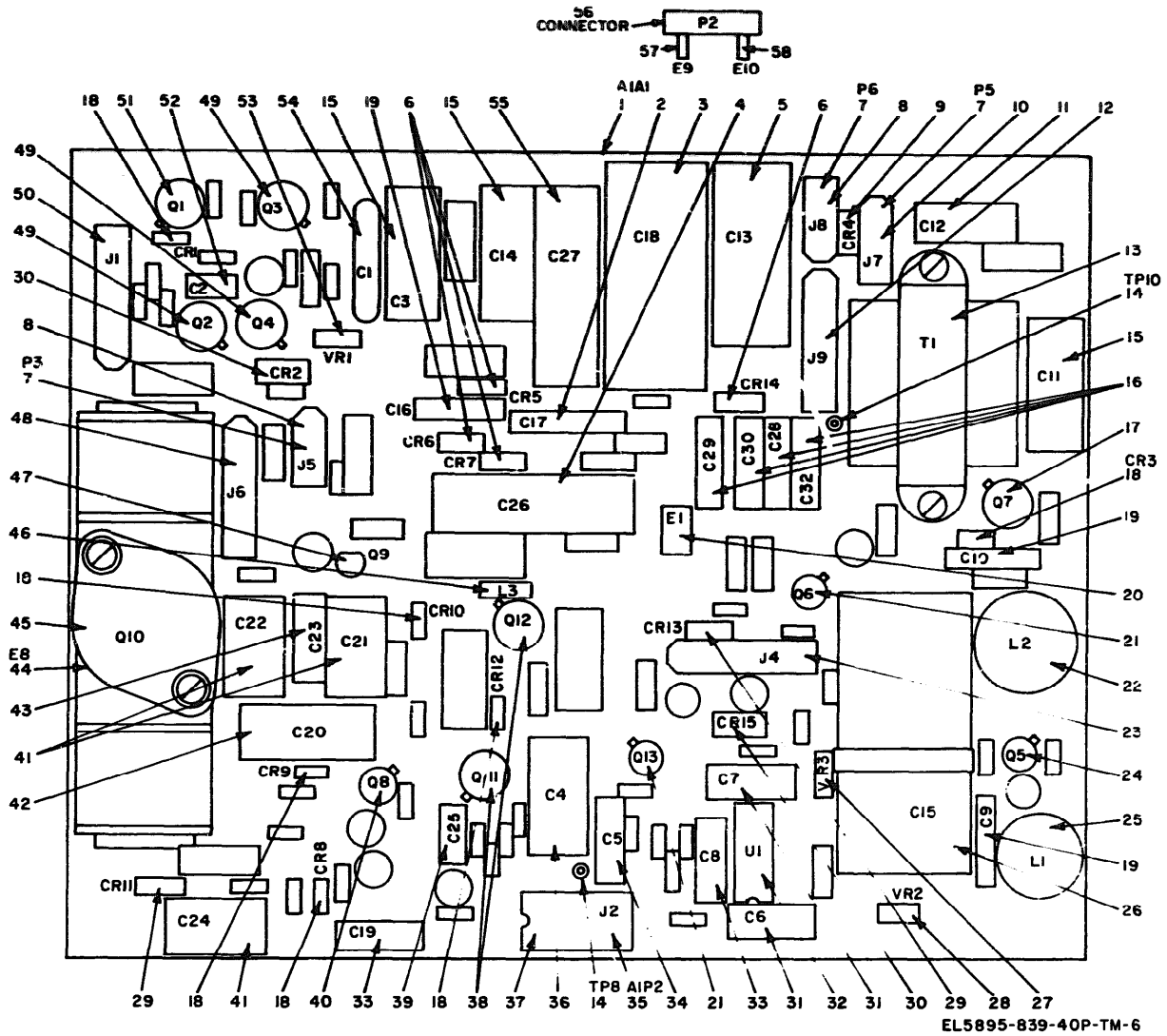
Figure 6. Circuit card assembly, 398-14939-1 (video and deflection), parts location.
