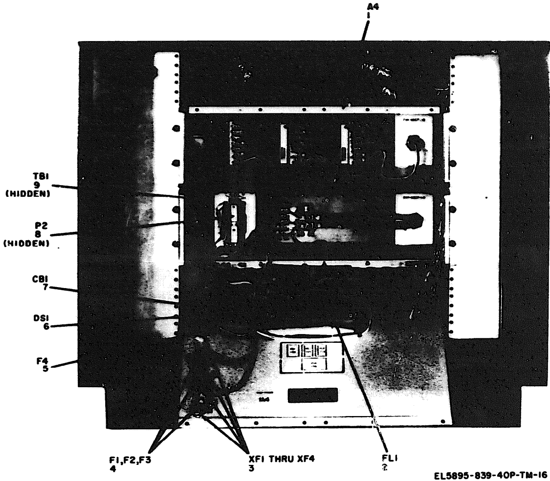
Figure 16. Power supply assembly, 398-15370-1, parts location.
