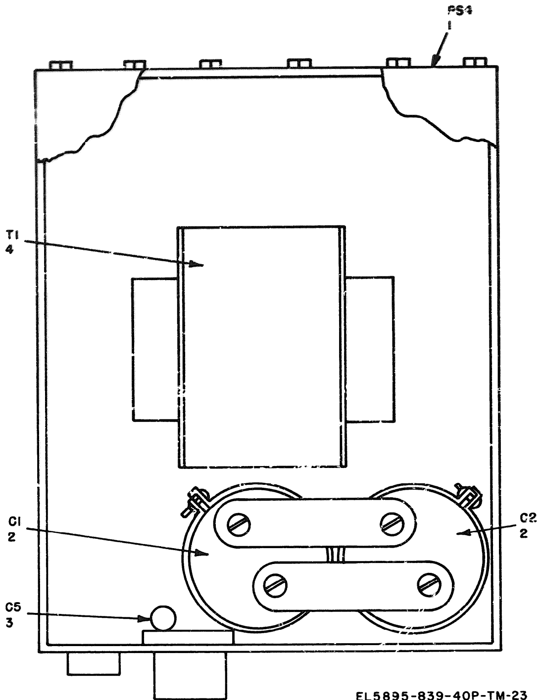
Figure 23. Power Supply PP-7144/U, top view, inside.
