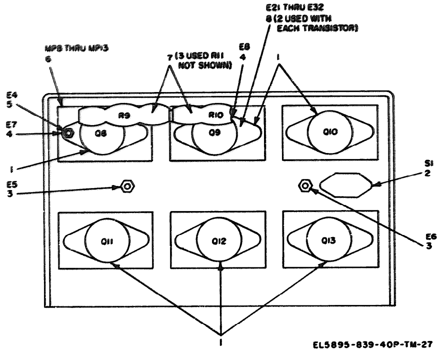
Figure 27. Power Supply PP-7144/U, rear view, inside.
