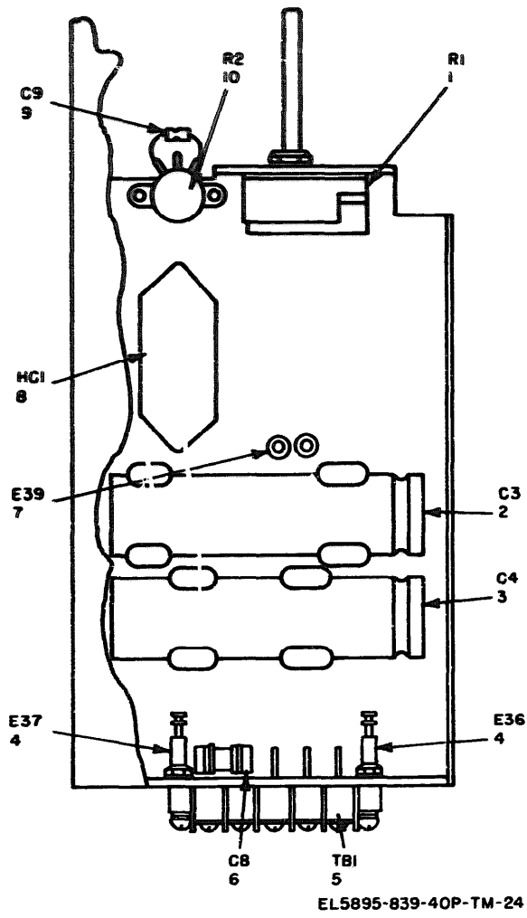
Figure 24. Power Supply PP-7144/U, left view, inside.
