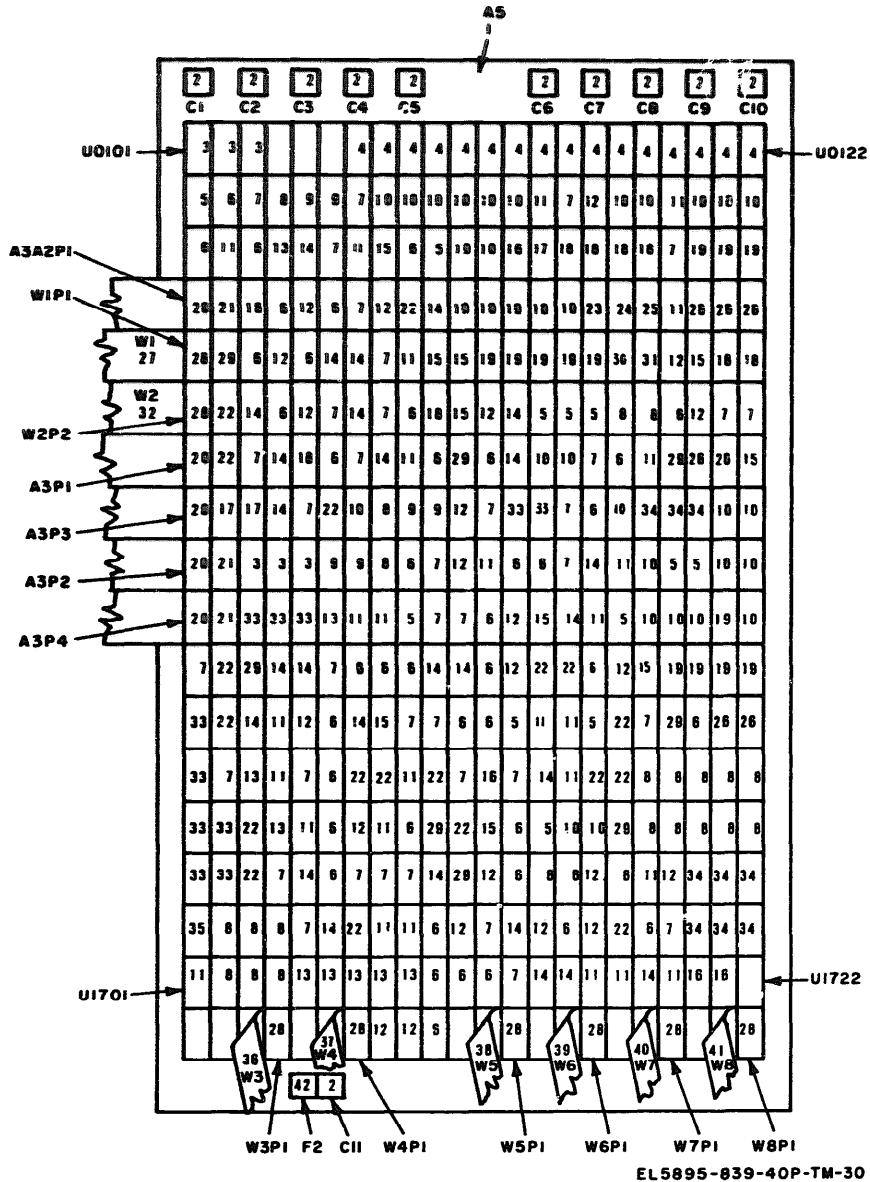
Figure 30. Interface and control logic panel, 398-15371-2, parts location.
