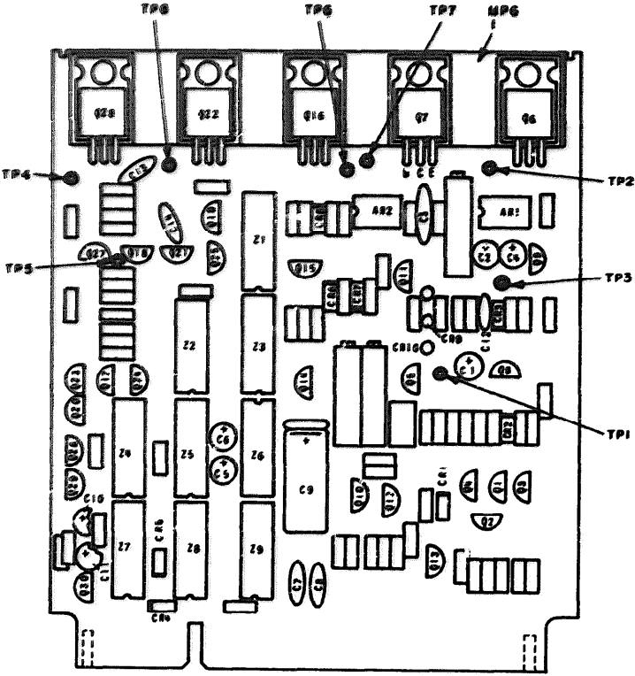
Figure 11. Circuit card assembly 8500002-001 (motion control), component location
