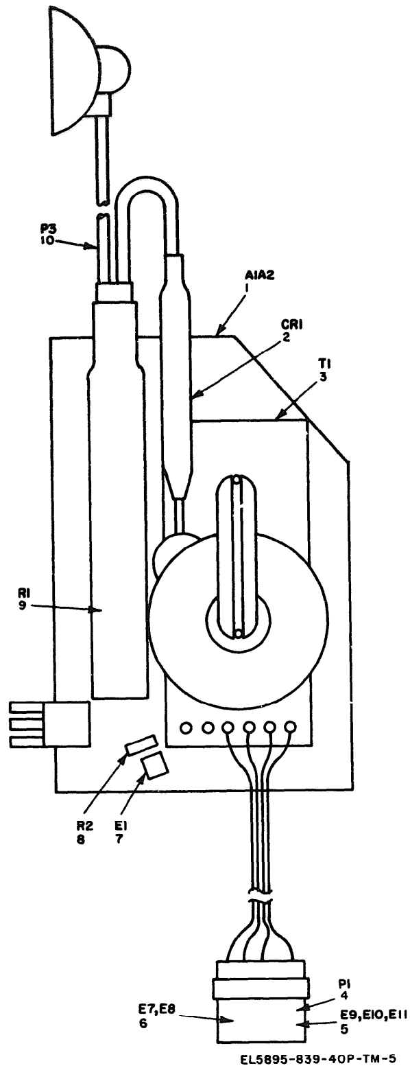
Figure 5. High voltage assembly, 398-14940-1, parts location.
