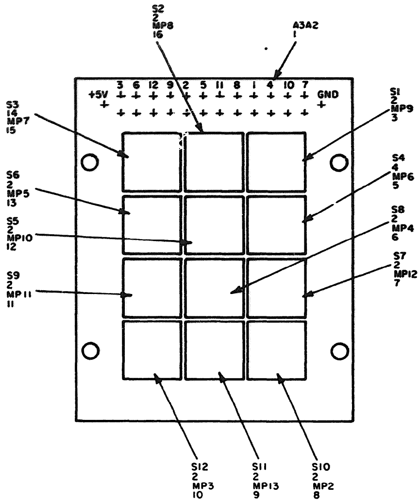
Figure 15. Keyboard subassembly 12SW3-33, parts location.
