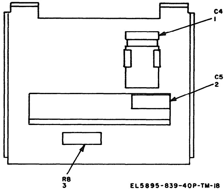
Figure 18. Power Supply PP-7145/U, rear view, inside.
