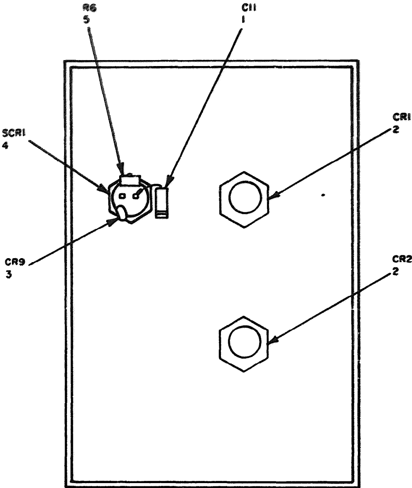
Figure 25. Power Supply PP-7144/U, front view, inside.
